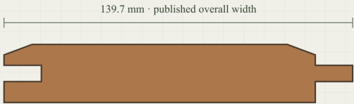
CROSS SECTION / PROFILE ILLUSTRATION
