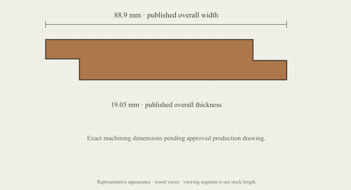
CROSS SECTION / PROFILE ILLUSTRATION
