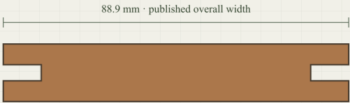
CROSS SECTION / PROFILE ILLUSTRATION
